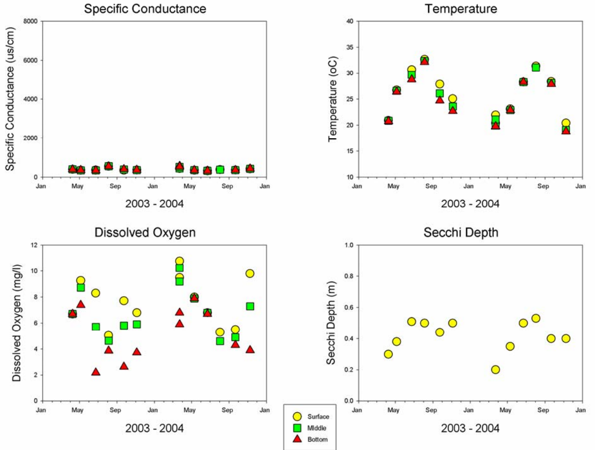
Figure 50.—Water column profile physicochemical parameter data at three depths and Secchi depth in Lost River at station LR 1, at the Chambers County line and 5.4 km upstream of John Wiggins Bayou.
